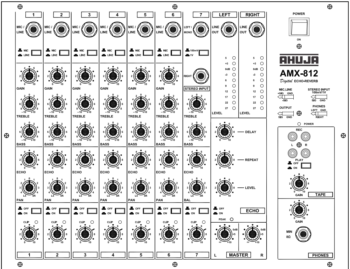
TOP PANEL
