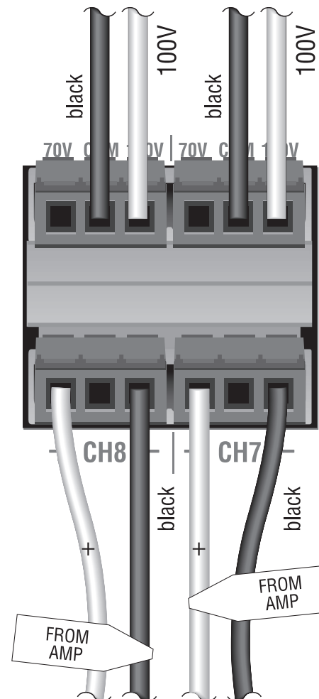
Figure 2. 100V Output
