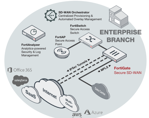
FortiGate 200F Enterprise Branch Deployment (Secure SD-WAN)
